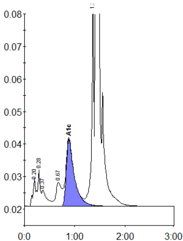
Peak table - ID: 10646700
